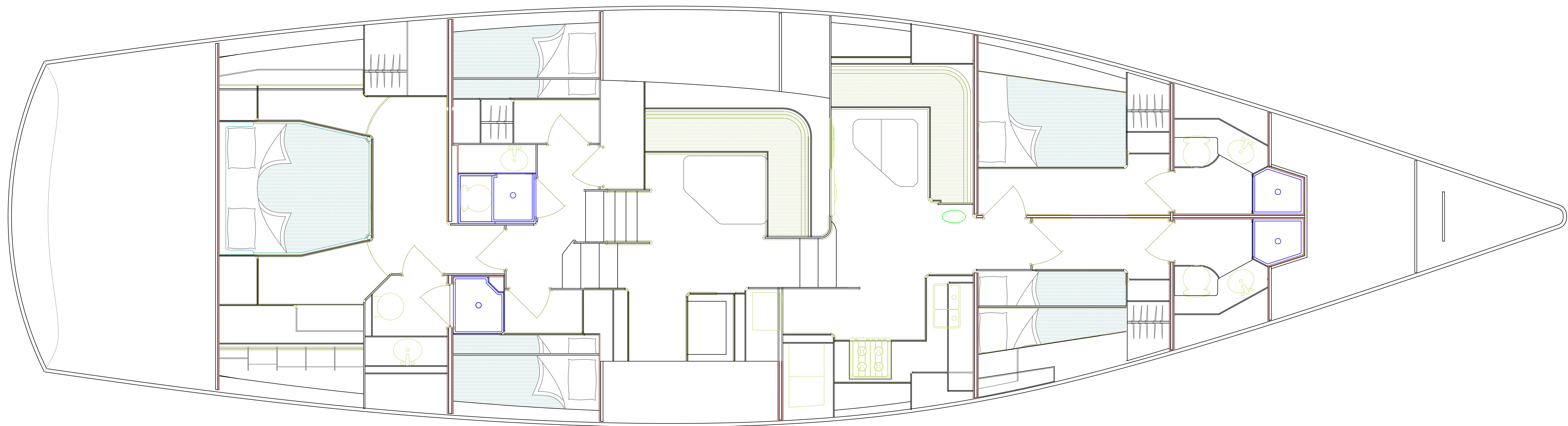
LYMAN MORSE DEERFOOT 70 INTERIOR ARRANGEMENT
